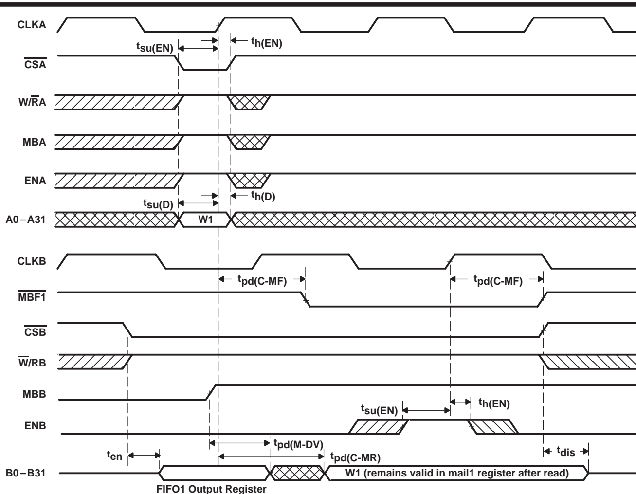
Figure 21. Timing for Mail1 Register and \overline{\text{MBF1}} Flag
