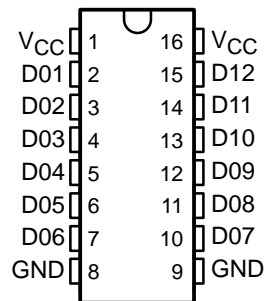
D, N, NS, OR PW PACKAGE (TOP VIEW)
