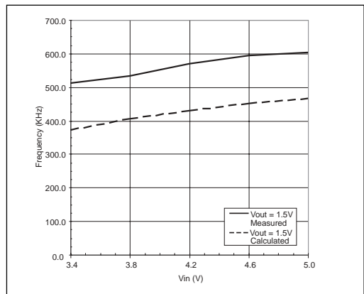
Ripple Frequency vs. V_{IN} , I_{OUT}=0.4A , V_{OUT}=1.5V
