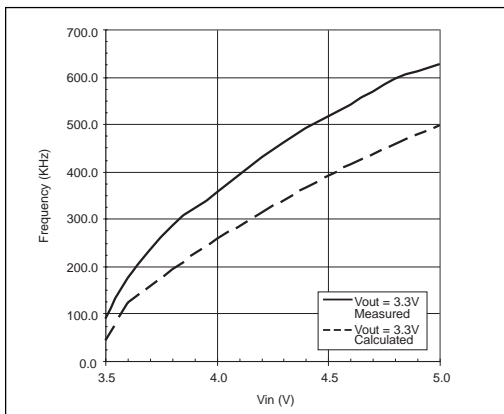
Ripple Frequency vs. V_{IN} , I_{OUT}=0.4A , V_{OUT}=3.3V
