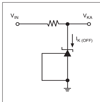
Figure 4. Test Circuit for I_{KOFF}
