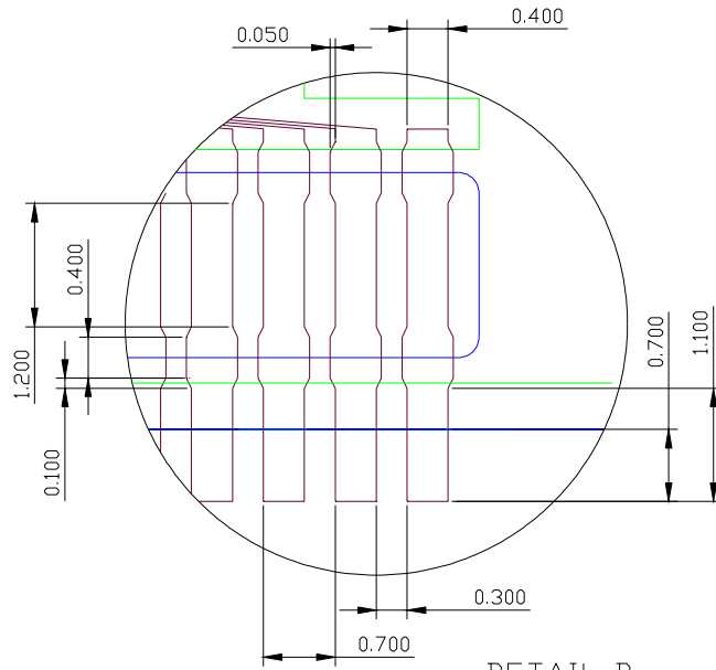
DETAIL B
