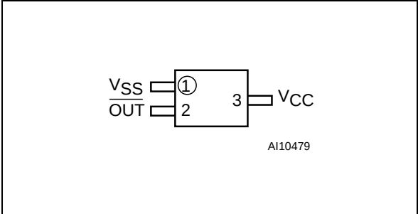
Figure 4. SOT323-3 (SC70-3) Connections
