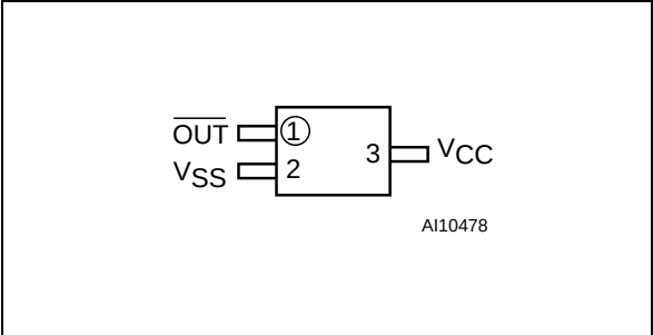
Figure 3. SOT23-3 Connections
