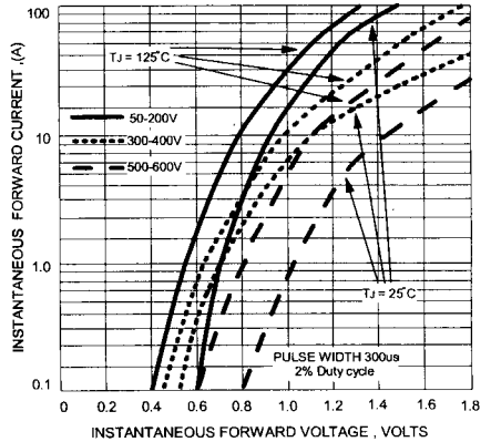
FIG. 4 - TYPICAL FORWARD CHARACTERISTICS
