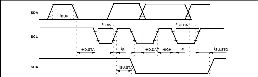
Figure 19. I²C Bus Timing
