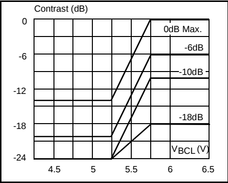
Figure 16. Automatic RGB Peak Regulation (APR) / RGB Peak Limitation Characteristics
