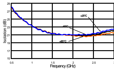
Isolation vs. Frequency, Over Temperature, 39 pF
