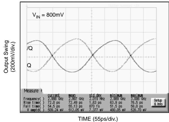
TIME (55ps/div.)
