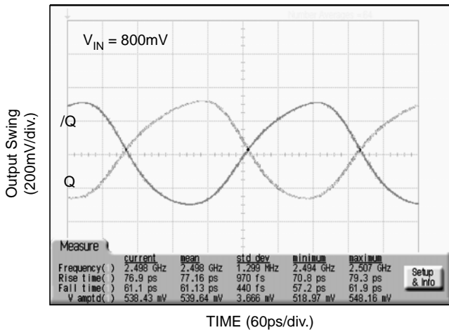
TIME (60ps/div.)
