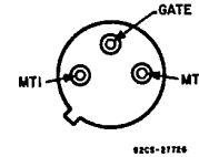
Modified TO-205
