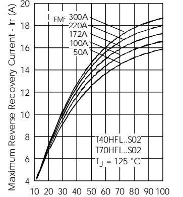
Rate Of Fall Of Forward Current - di/dt (A/µs)
