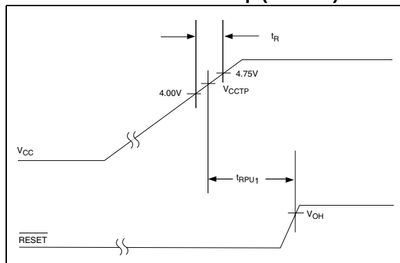
FIGURE 3-1: Timing Diagram – Power Up (TC1279)
