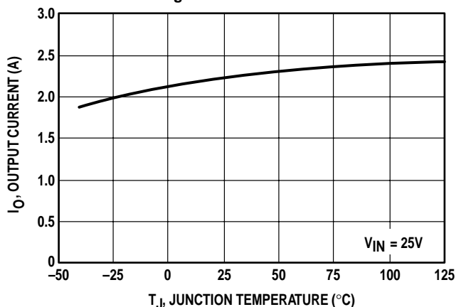
Figure 23. Current Limit
