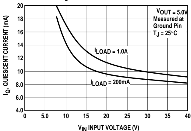
Figure 25. Quiescent Current
