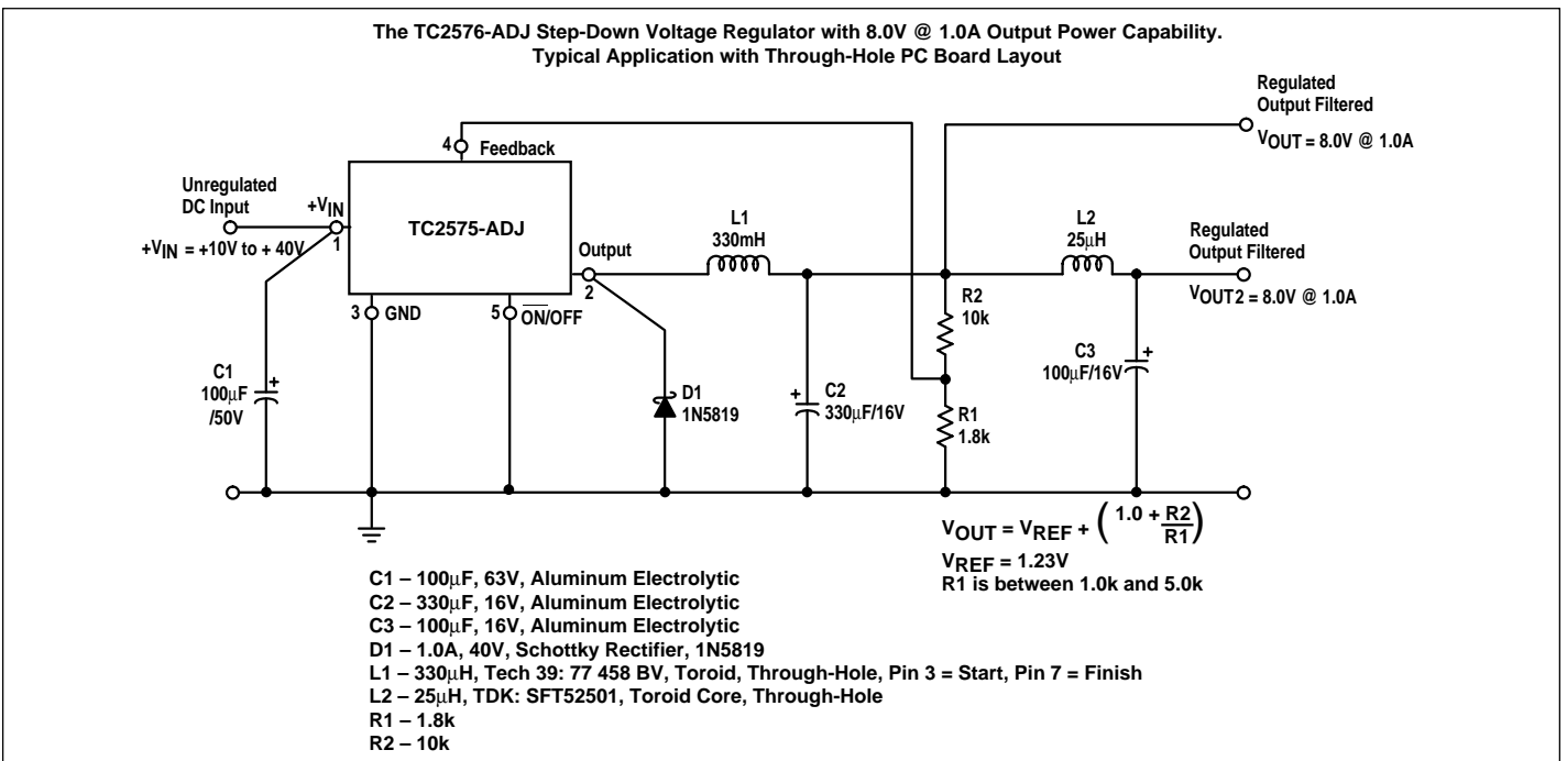
Figure 17. Schematic Diagram of the 8.0V @ 1.0A Step-Down Converter Using the TC2575-ADJ
