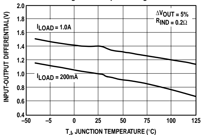
Figure 24. Dropout Voltage
