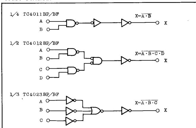
TC4023BP/BF
