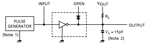
8. t_{ON}, t_{OFF}
