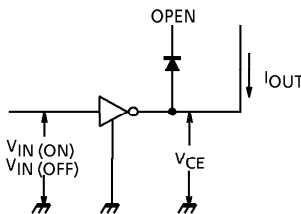
5. V_{IN(ON)}, V_{IN(OFF)}
