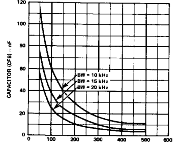
CAPACITOR (CFB) AS A FUNCTION OF GAIN (VARIOUS BANDWIDTHS)
