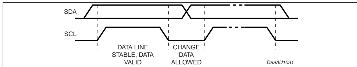
Figure 29. Timing Diagram on the I 2 C BUS
