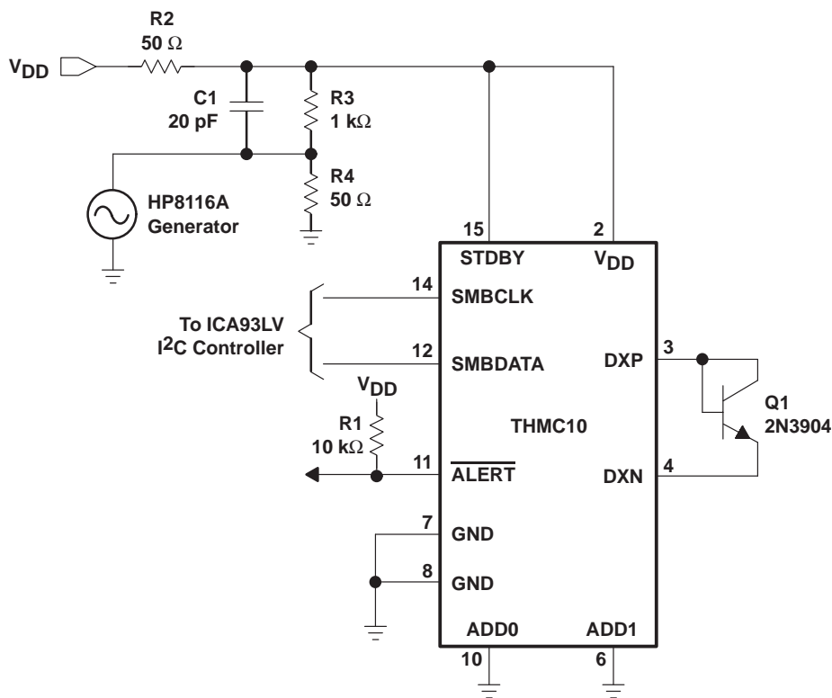
Figure 10. Test Circuit
