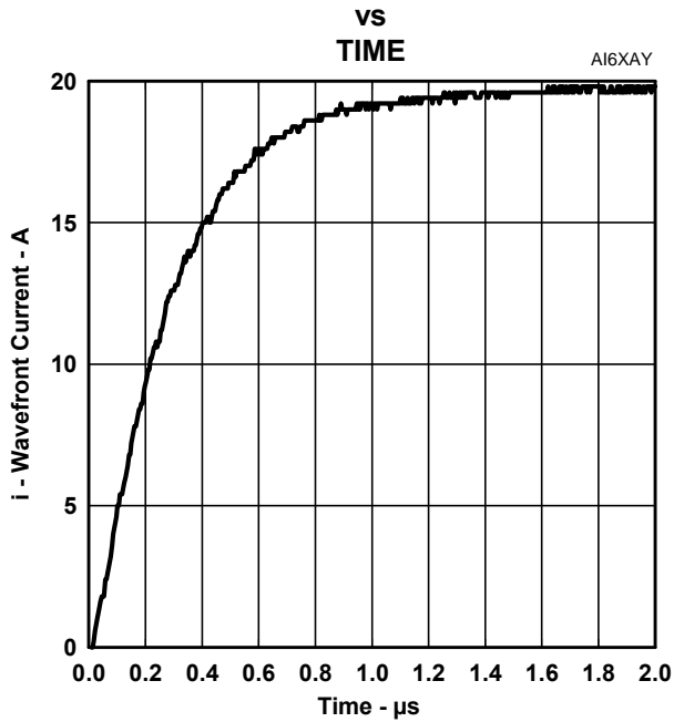
Figure 4. CURRENT WAVEFRONT
