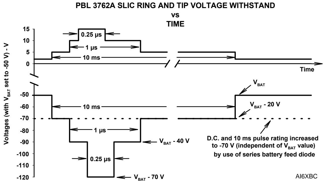
Figure 15. TRANSIENT LIMITS FOR PBL 3762A WITHSTAND VOLTAGE
