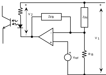
FIGURE 2: ERROR AMPLIFIER / OPTO-COUPLER COMBINATION
