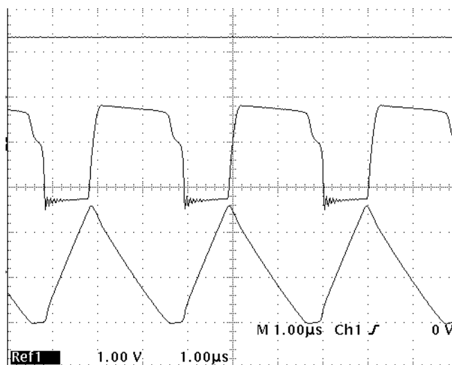
FIGURE 1: CHARACTERISTIC WAVEFORMS OF THE TK75002
