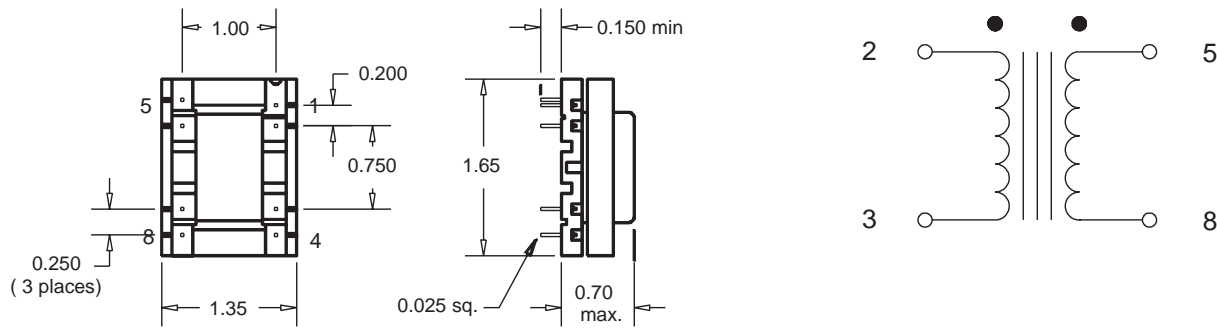
All dimensions are in inches
