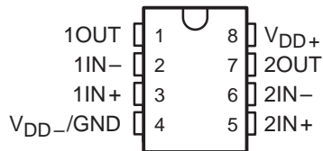
TLC2252M, TLC2252AM ... JG PACKAGE (TOP VIEW)
