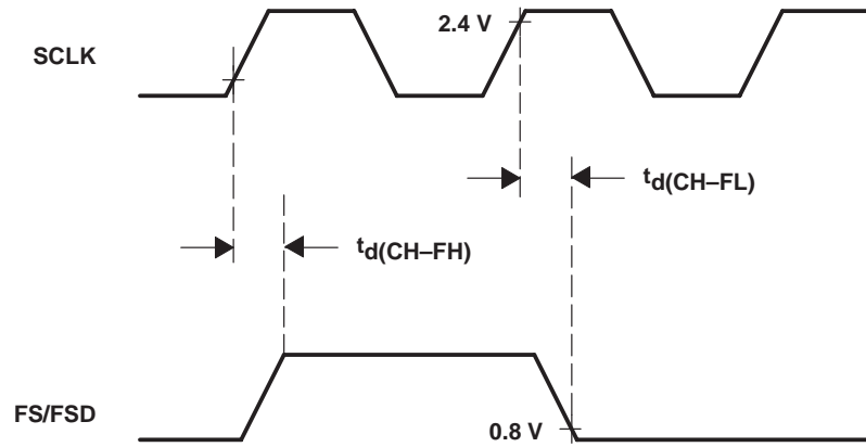
Figure 5-1. FS and FSD Timing
