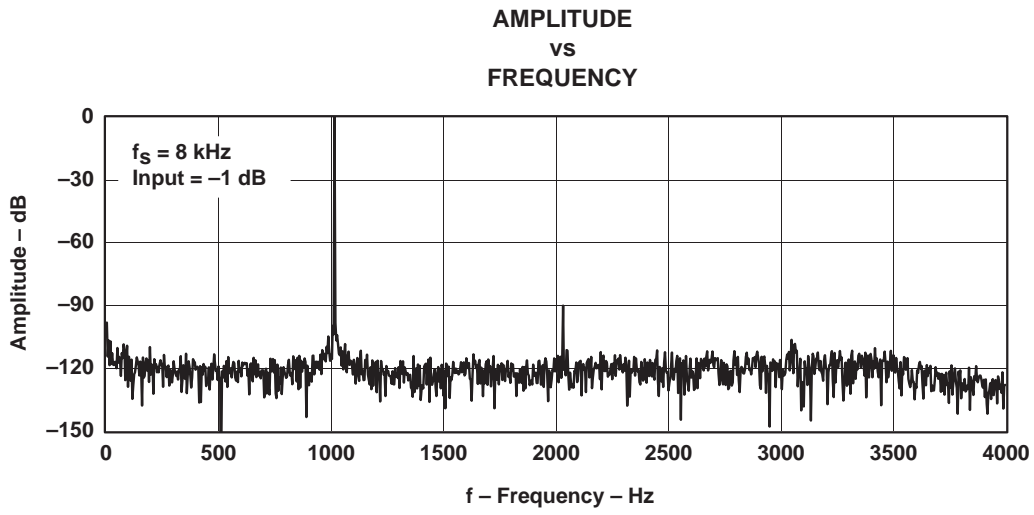
Figure 5-7. FFT-ADC Channel, f_s = 8 \text{ kHz} , Input = -1 dB
