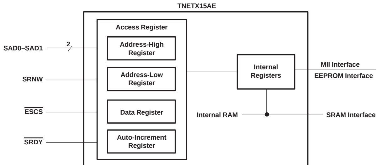
Figure 2. DIO Access (Pointer) Registers
