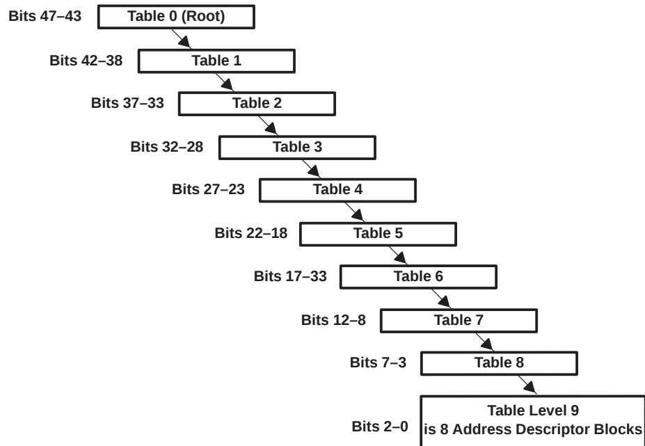
Figure 10. Address Tables
