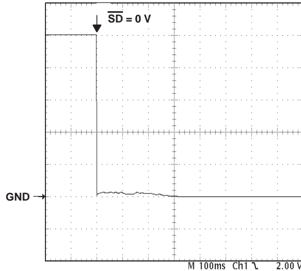
Figure 45. Differential Output With FADE Terminal Held High
