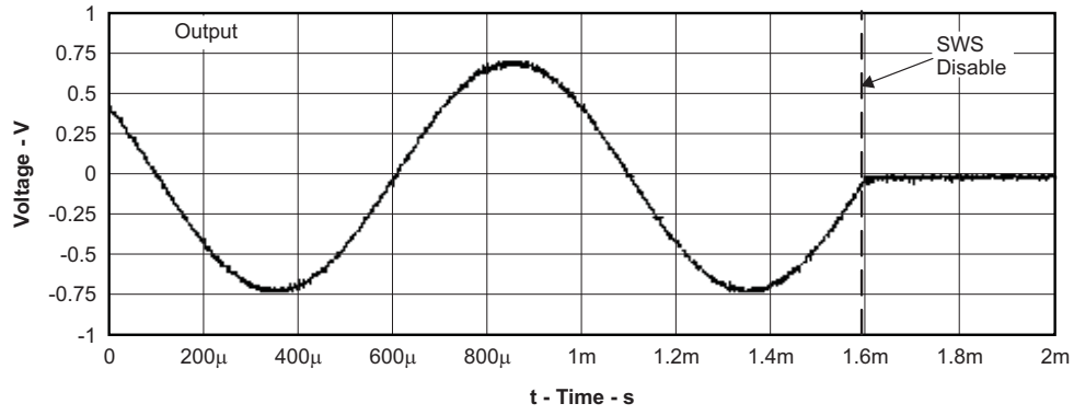
Figure 34. Shutdown Time
