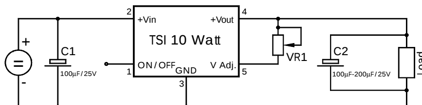
Output Voltage Adjustment Connection
