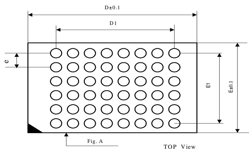
48 Mini-BGA 6*8mm
