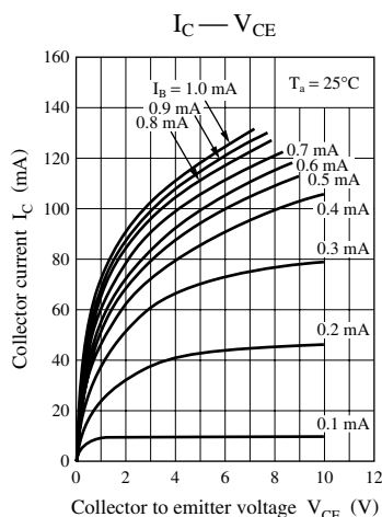
Characteristics chart of UNR9211J
