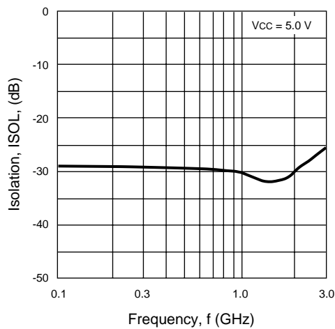
UPC2711TB ISOLATION vs. FREQUENCY
