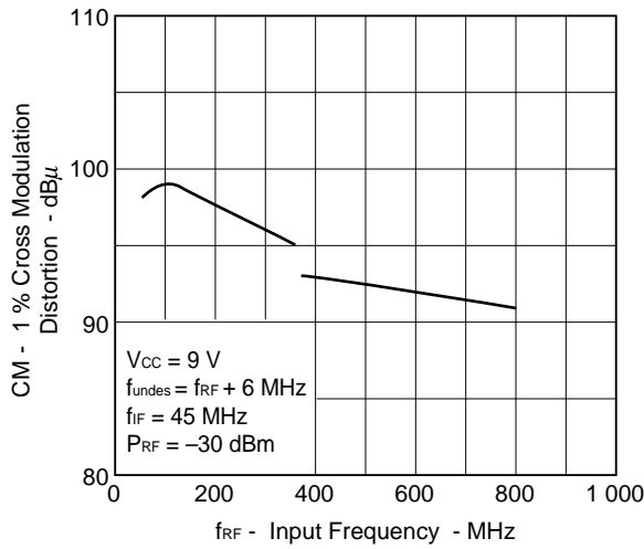
CM vs. f_{RF}
