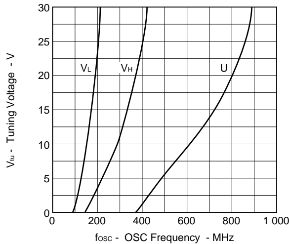
V_{tu} vs. f_{osc}
