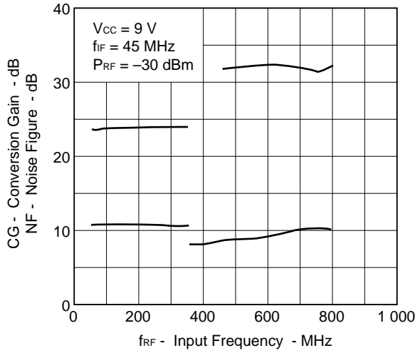
CG, NF vs. f_{RF}
