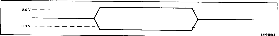
Figure 3. Output Timing
