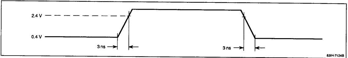
Figure 3. Output Timing
