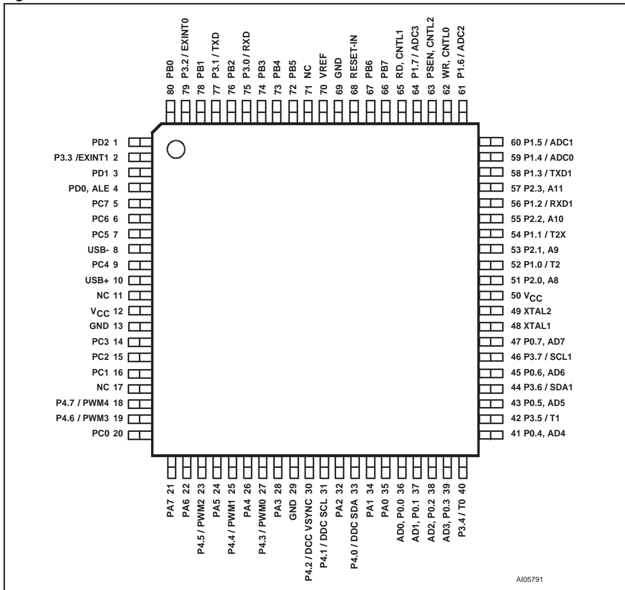
Figure 4. TQFP80 Connections
