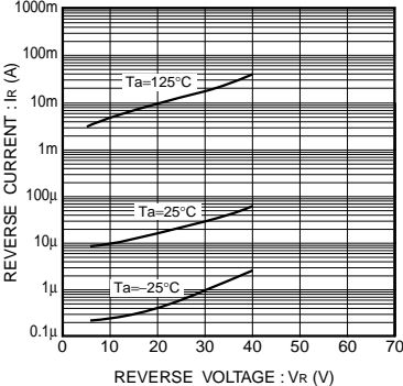
Fig.09 Reverse characteristics
