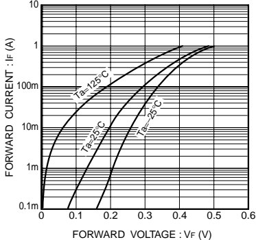
Fig.8 Forward characteristics
