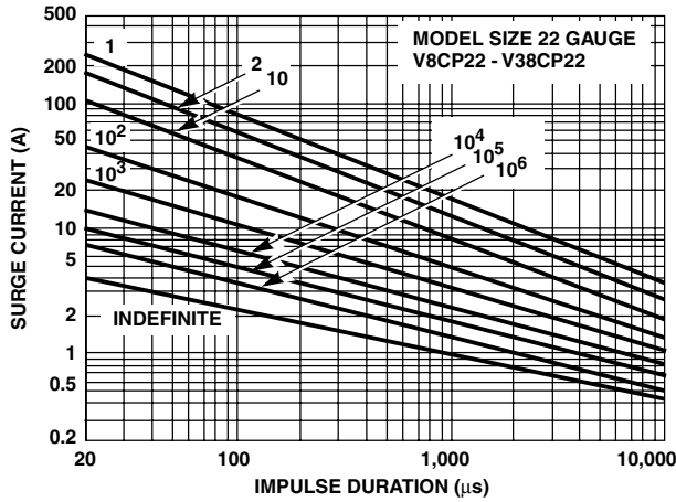
FIGURE 15. SURGE CURRENT RATING CURVES FOR V8CP22 - V38CP22
