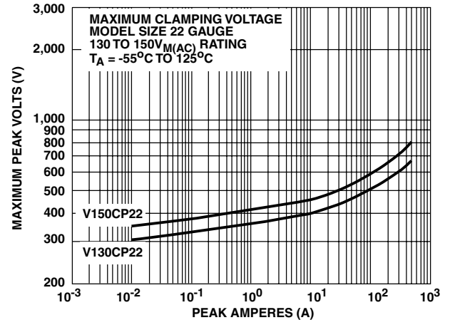
FIGURE 8. CLAMPING VOLTAGE FOR V130CP22 - V150CP22
