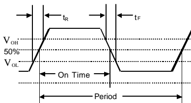
Figure 1. Output Waveform
