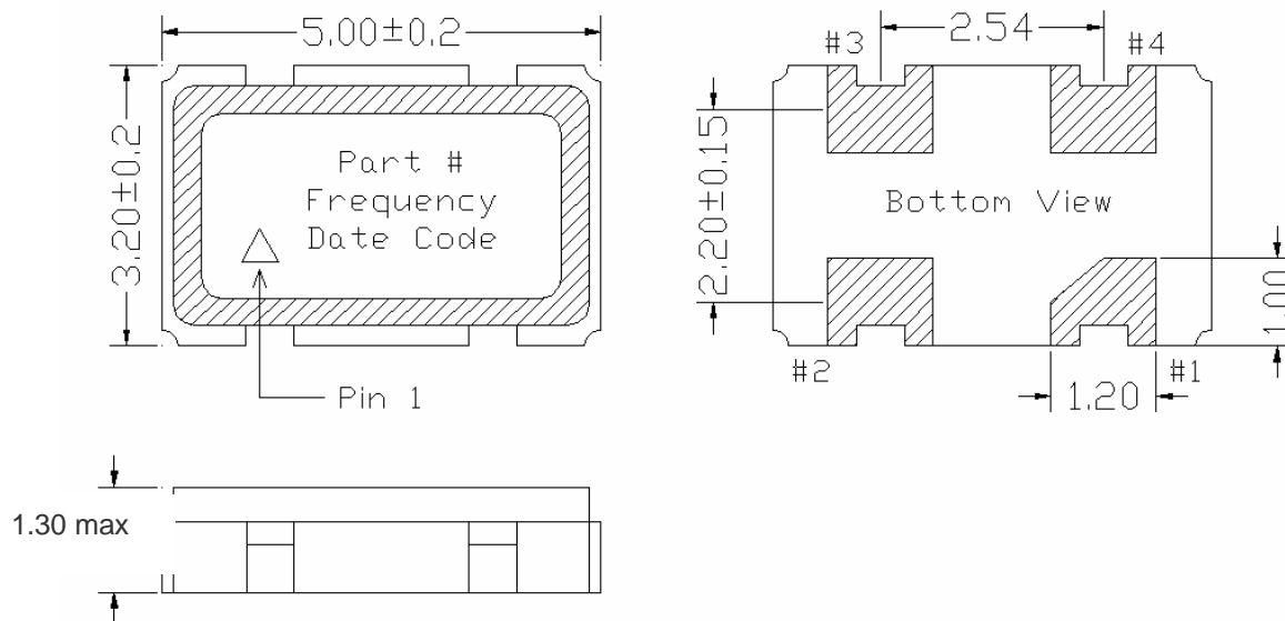
Figure 9, Package drawing
