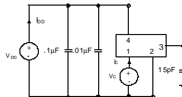
Figure 8. Typical Output Test Conditions (25±5°C)
