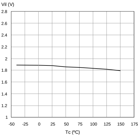
Figure 21. Input Low Level
