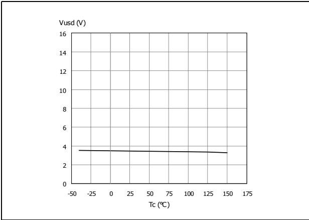
Figure 19. Undervoltage shutdown
