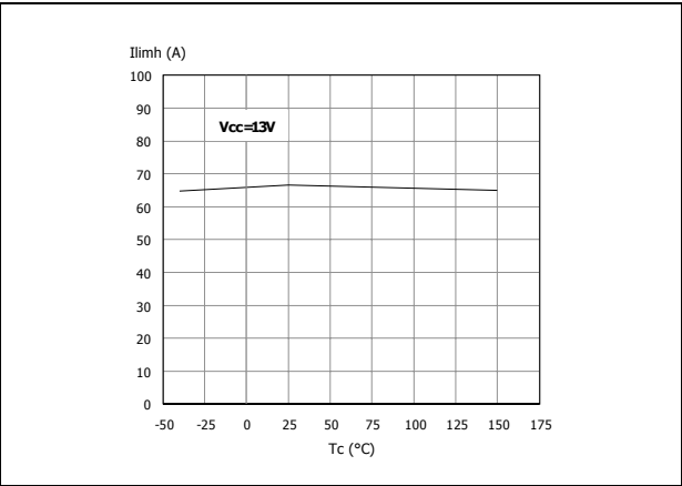
Figure 20. I_{LIMH} vs T_{case}
