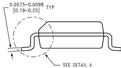
SEE DETAIL A
