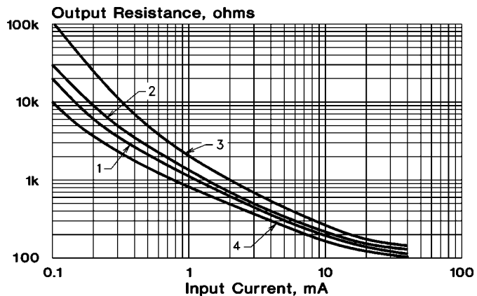
Output Resistance vs. Input Current VTL5C4/2
