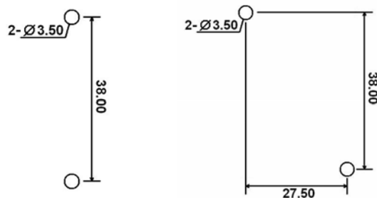
FLANGE MOUNT LAYOUTS
