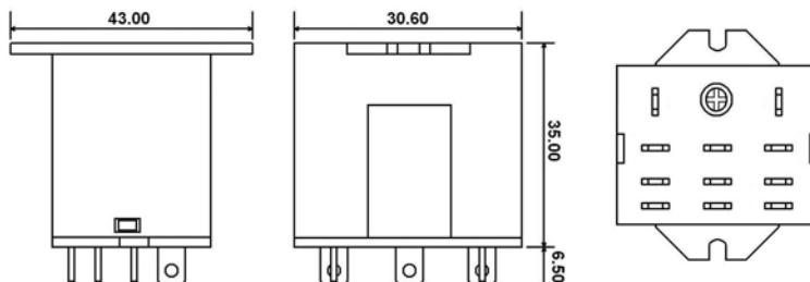
3 POLE WITH FLANGE
