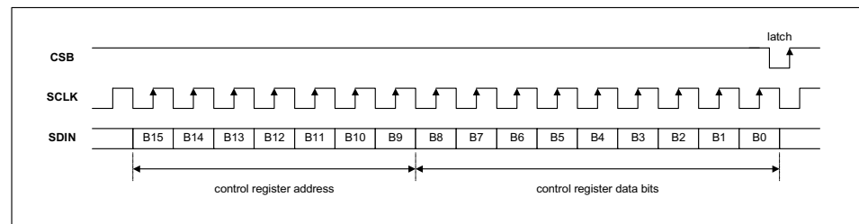
Figure 21 3-Wire Serial Control Interface
