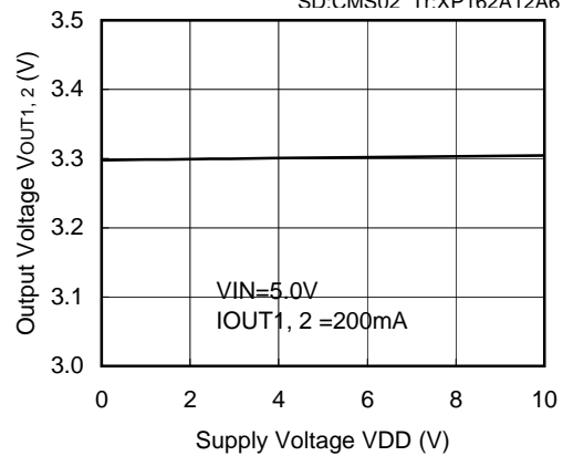
XC9503B093(300kHz)
