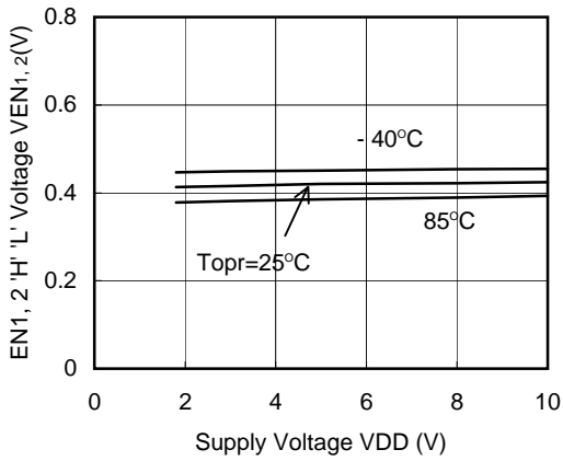
XC9503B093 (300KHz)
