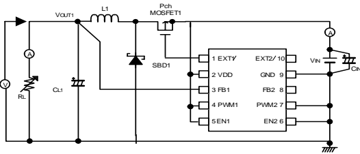
Circuit 3
