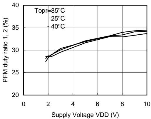
XC9503B093(300kHz)
