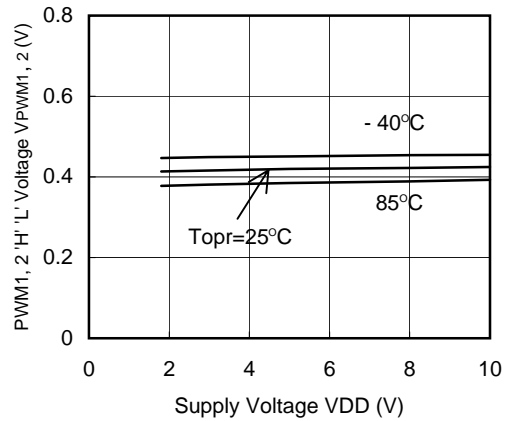
XC9503B093 (300KHz)
