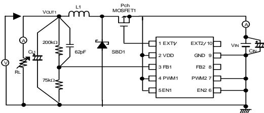
Circuit 4
