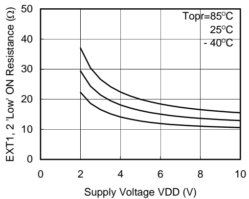
XC9503B092 (180KHz)
