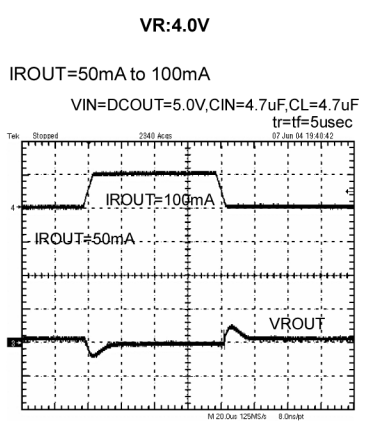
VR: 50mV/div Time: 20usec/div
