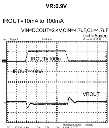
VR: 50mV/div Time: 20usec/div
