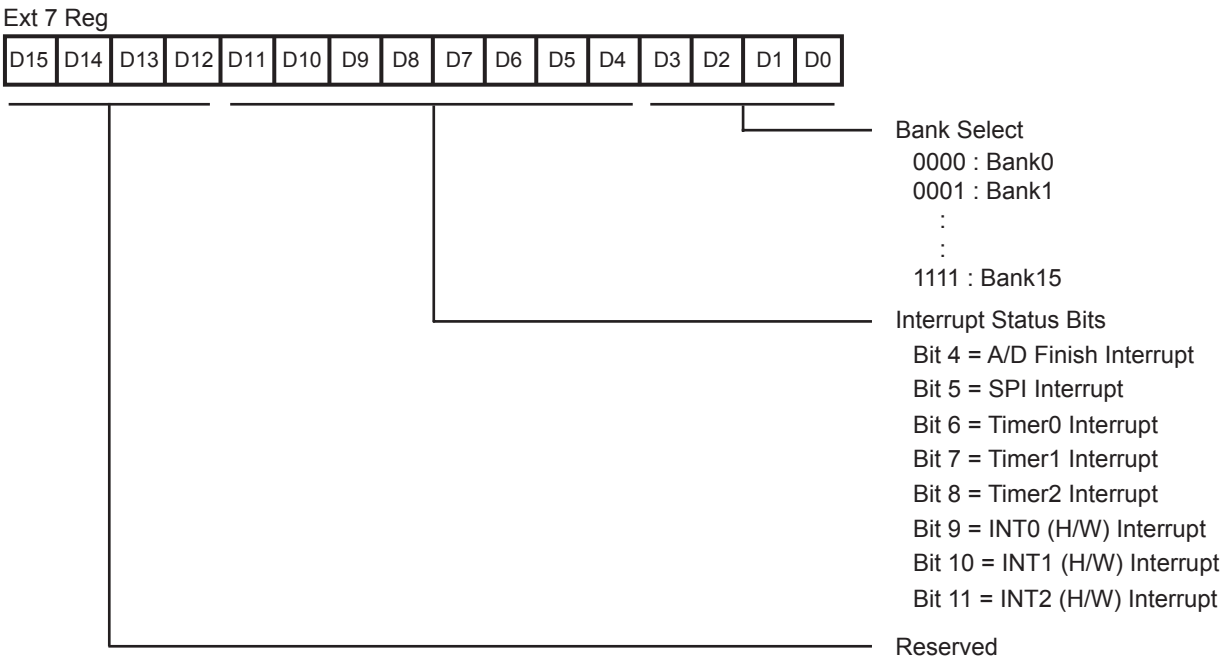
Figure 20. EXT7 Register
