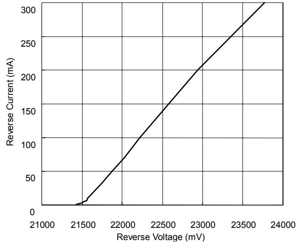
ZD5251B Reverse Current vs Reverse Voltage
