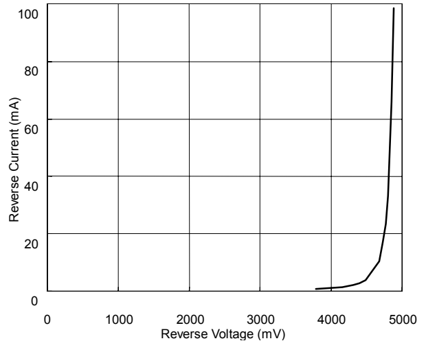
ZD5230B Reverse Current vs Reverse Voltage
