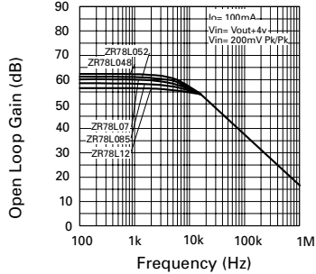
Ripple Rejection v Ripple Frequency
