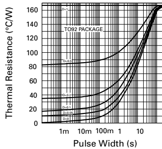
Thermal Resistance v Pulse Width
