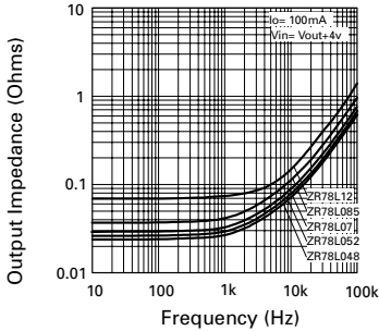
Output Impedance v Frequency
