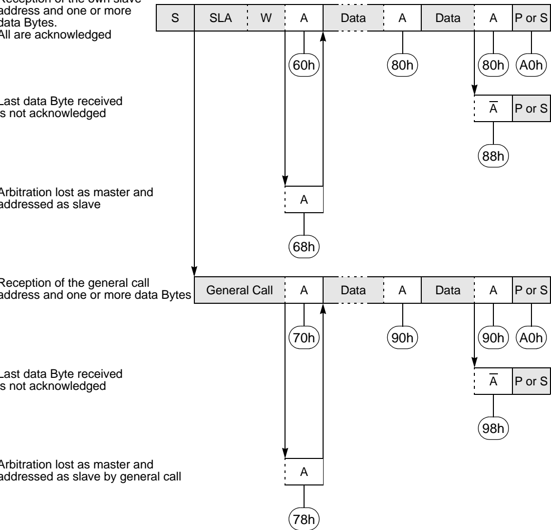
Figure 134. Format and States in the Slave Receiver Mode
