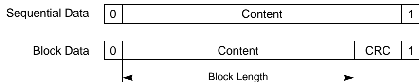
Figure 88. Data Token Format
