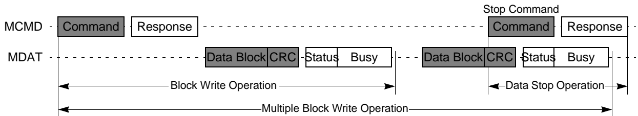
Figure 84. Multiple Block Write Operation
