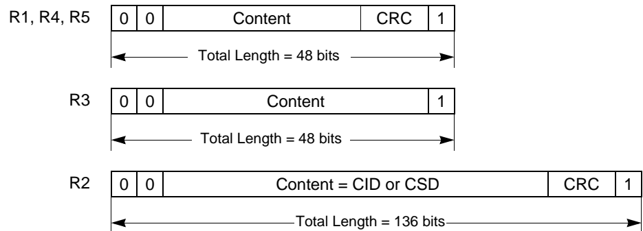
Figure 87. Response Token Format
